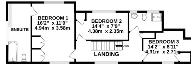
1ST FLOOR 687 sq.ft. (63.8 sq.m.) approx.
