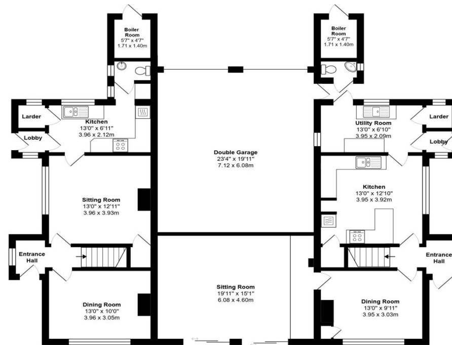
Ground Floor
